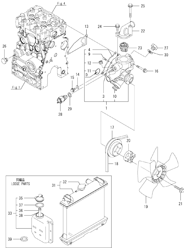
Fig.9. COOLING WATER SYSTEM
