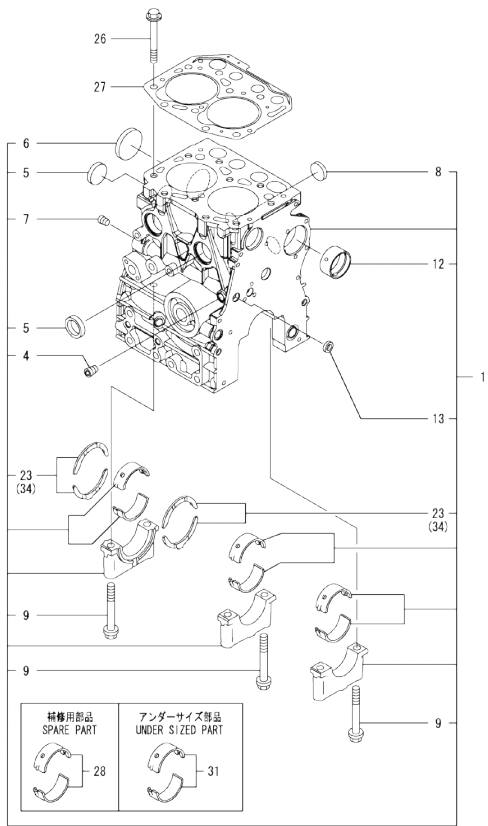
Fig.1. CYLINDER BLOCK
